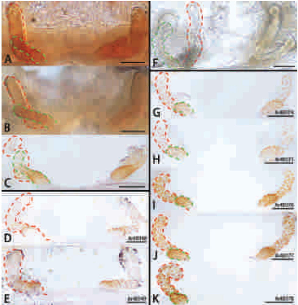
Figure 6. Ectatosticta spp., variation of female genitalia (red line, inner spermathecae (A–C, F–K) or spermathecae (D, E); green line, outer spermathecae) A–C E. deltshevi , females from Qinghai (type locality) D, E E. wukong sp. nov., paratypes F E. davidi , females from Shaanxi G–K E. xuanzang sp. nov., paratypes. Scale bars: 0.1 mm.
