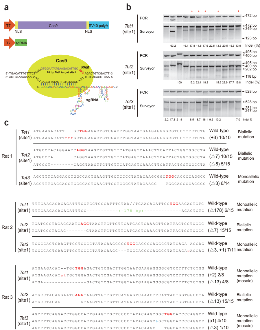
Figure 1 Targeted disruption in the Tet gene loci in rat by means of CRISPR-Cas systems. (a) Engineered CRISPR-Cas systems and their target Tet1 gene locus used in this study. The protospacer adjacent motif (PAM) is shown in red letters, and the 20-base-pair spacer sequence is shown in purple letters. NLS, nuclear localization signal. (b) The PCR products encompassing the targeted sites and their Surveyor assay for indels in the PCR products. All three Tet genes of each rat are assayed and presented in the same order. Individuals with heteroduplex of wild-type (WT) and mutated alleles have three bands in Surveyor assay, individuals with large indels have PCR and Surveyor products with shifted sizes. Indel rate is calculated and labeled under the lanes with mutation. *, rats with mutations in all three target sites. (c) Sanger sequencing of targeted gene alleles in each of the triple-mutated rats induced by injection of Cas9 enzyme together with sg Tet1 -1/sg Tet2 -1/sg Tet3 -1. The PAM sites are red, upper case bold; insertions are red, lower case; point mutations are blue, lower case. The sizes of the point mutations (p), insertions (+) or deletions (Δ) are shown to the right of each allele. The fractions indicate the read number of the mutant allele (numerator) out of total read number (denominator). The targeted locus is labeled as “biallelic mutation” if no wild-type allele reads were recovered, as “monoallelic mutation” if a wild-type allele was recovered, and as “mosaic” if more than two types of alleles were recovered (Supplementary Discussion).
